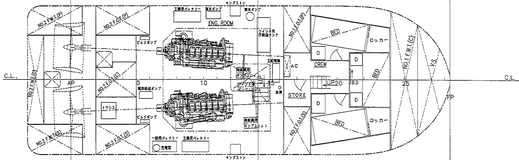
BOTTOM PLAN
